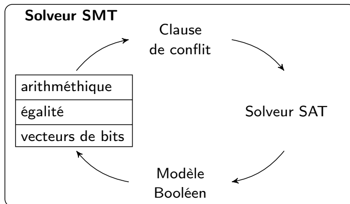
FIGURE 1.1 – Architecture d'un solveur SMT.
